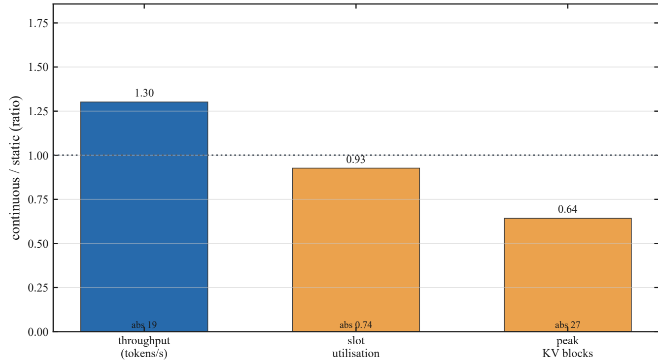
Continuous batching vs static batching (normalised) (GPU)
