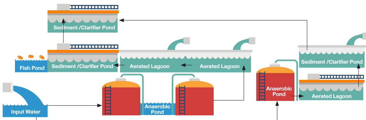
Figure : 1 Waste Water Treatment System
