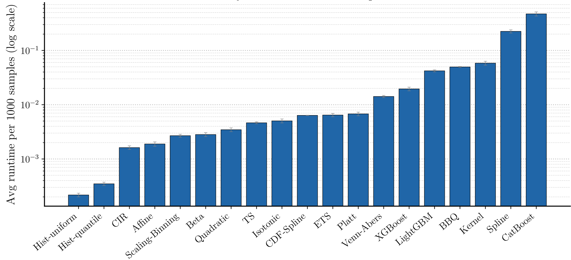
Binary methods runtime comparison
