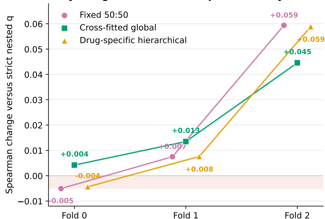
Only the global cross-fit improves every fold
