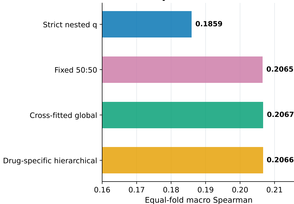
The three hybrids have the same mean
