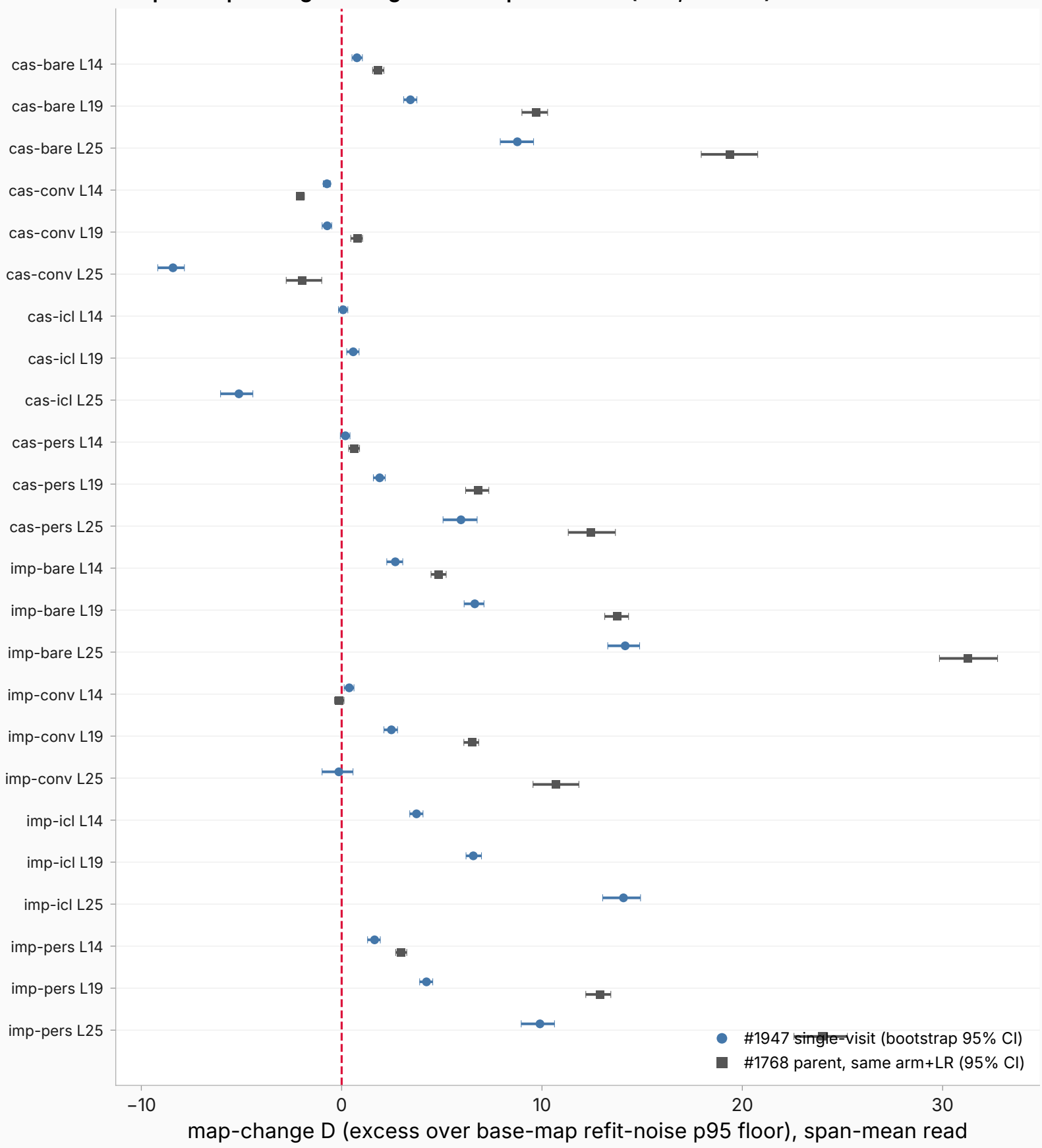
Corpus map-change D: single-visit vs parent fleet (n=3,000 fits)
