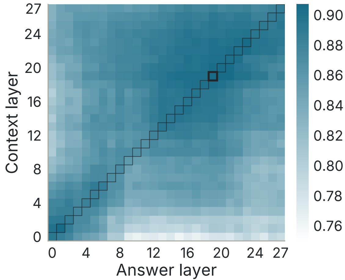
Top-1 retrieval of the ridge map
