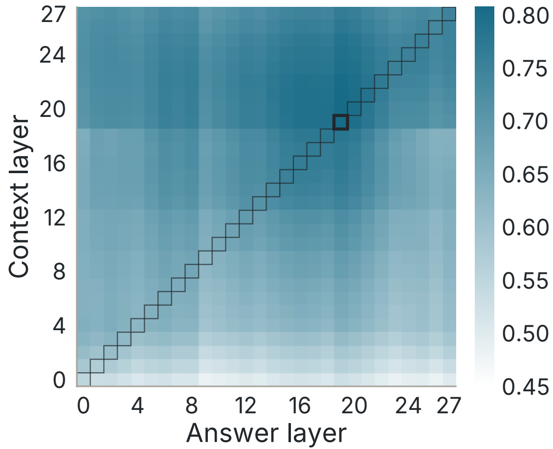
Held-out R^2 of the ridge map
