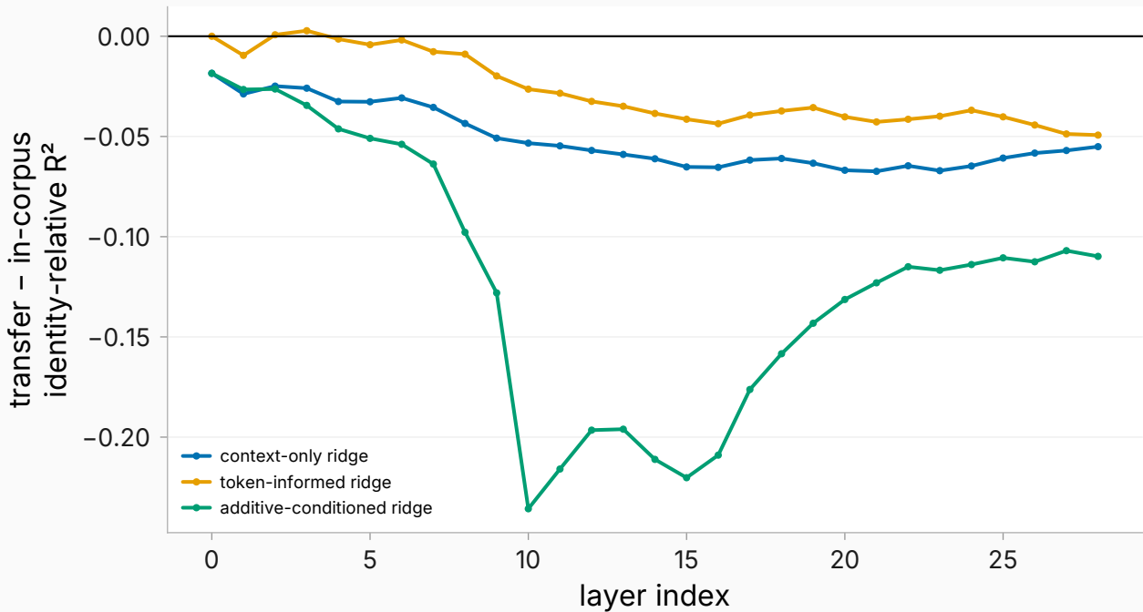
LMSYS→eval-condition transfer delta (single-step)
