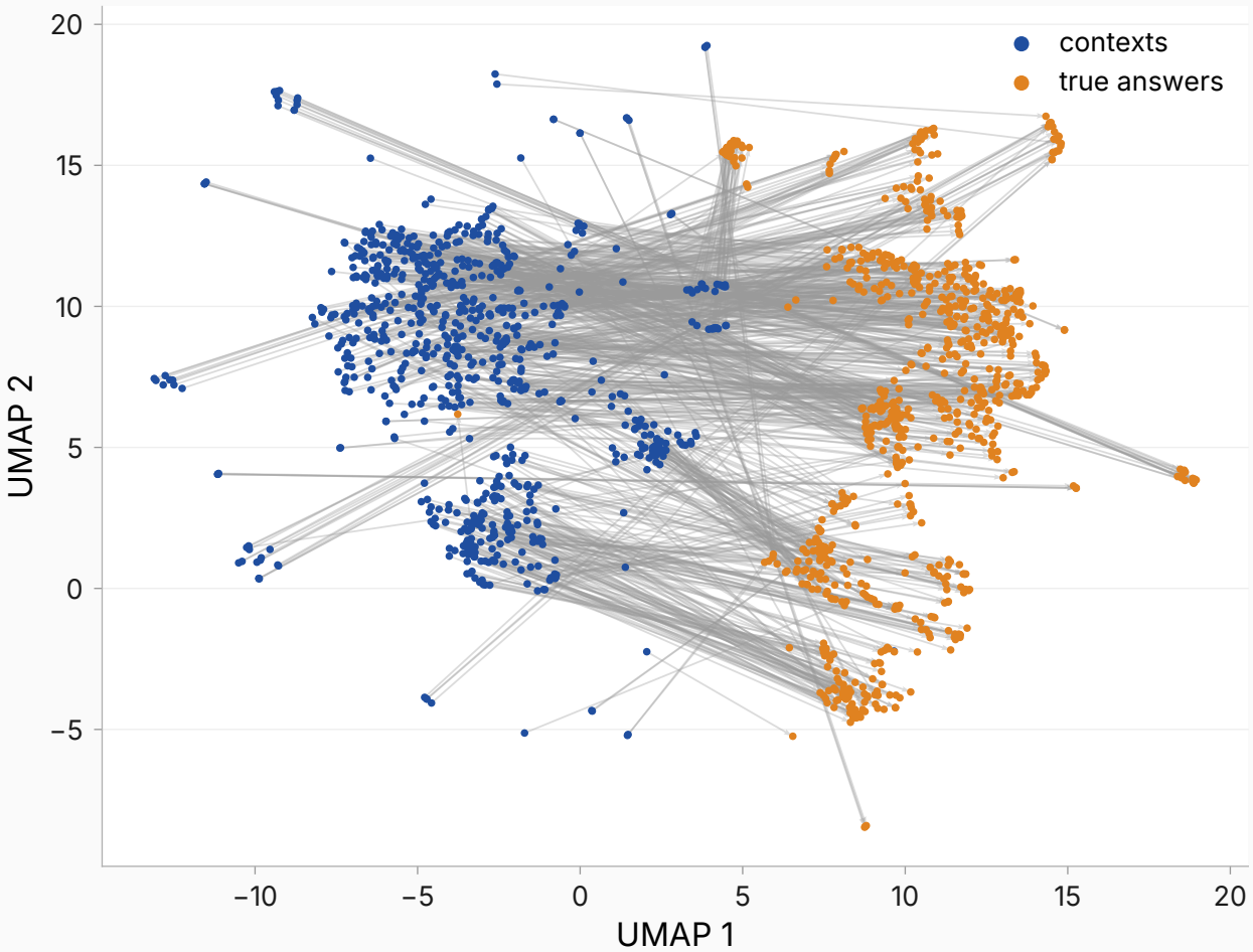
context → true-answer pairings (800 random pairs, seed 42)
