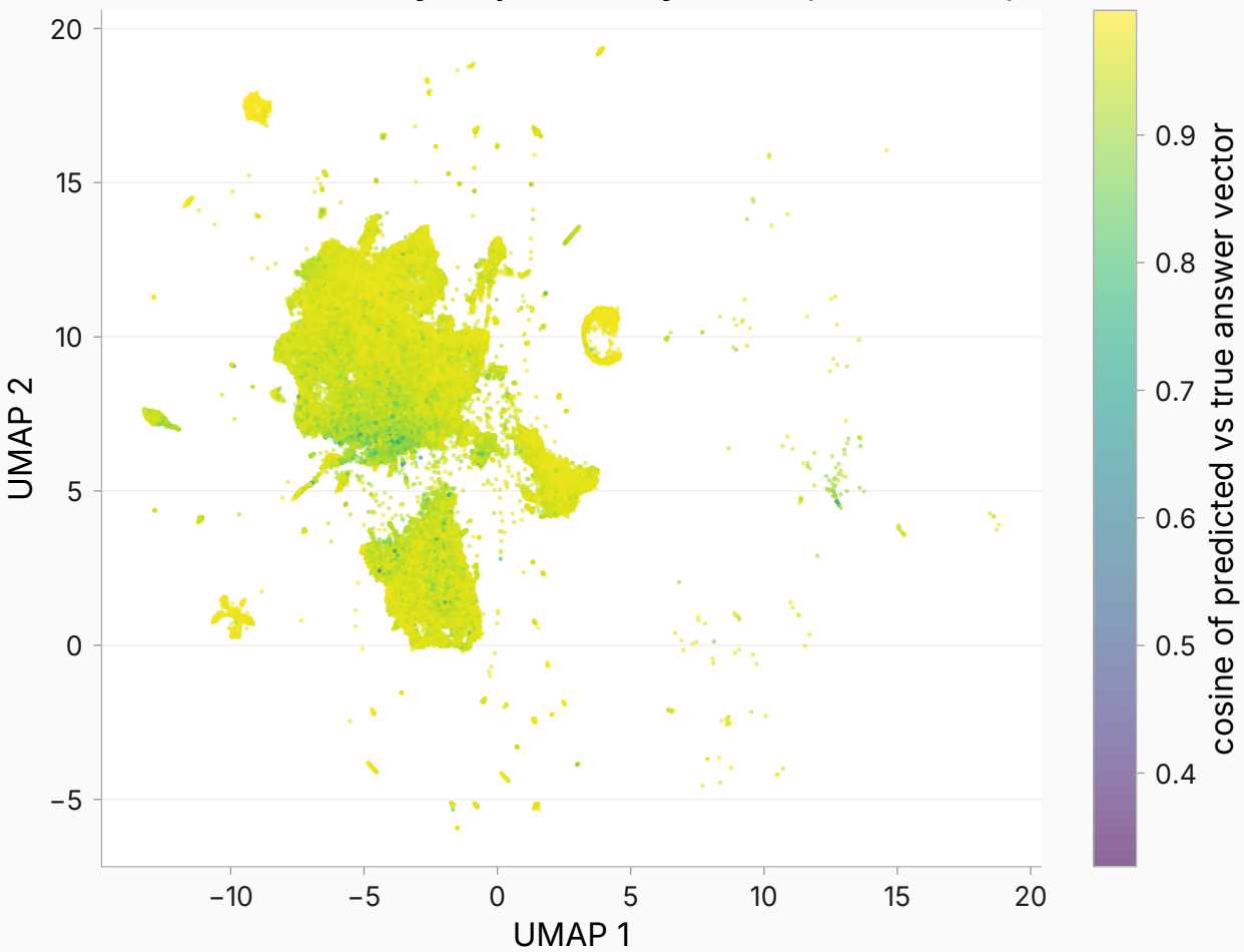
contexts colored by map accuracy (n=150,000 of 959,844)
