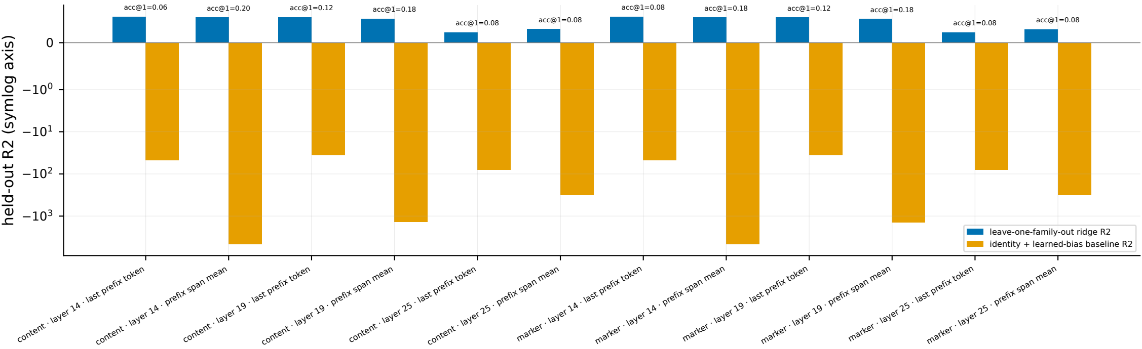
prefix-to-answer mapping fits (exploratory; n=50 < d=3584 regularization-limit regime)
