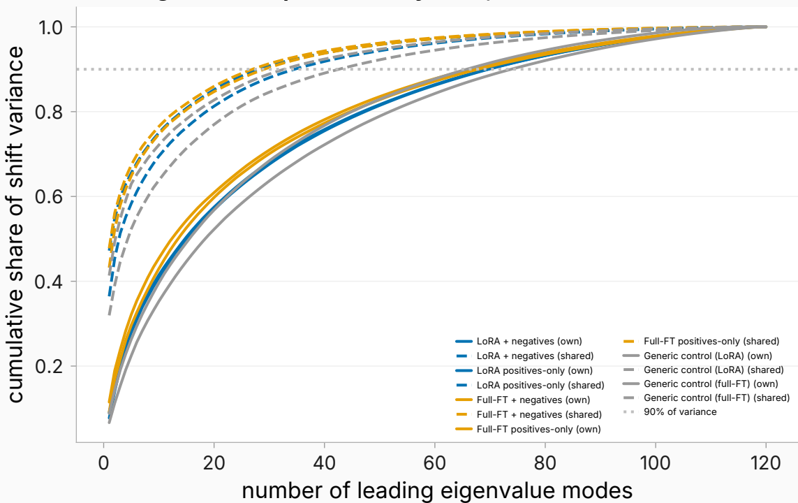
shift eigenvalue spectra — layer 14, own vs shared text
