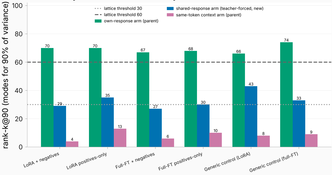
shift rank by measurement arm — layer 14 (shared text held fixed)
