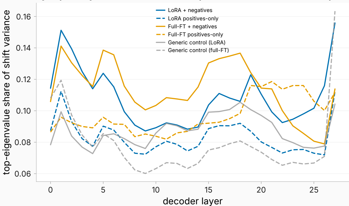
sycophancy activation shift — response arm (selected checkpoint)
