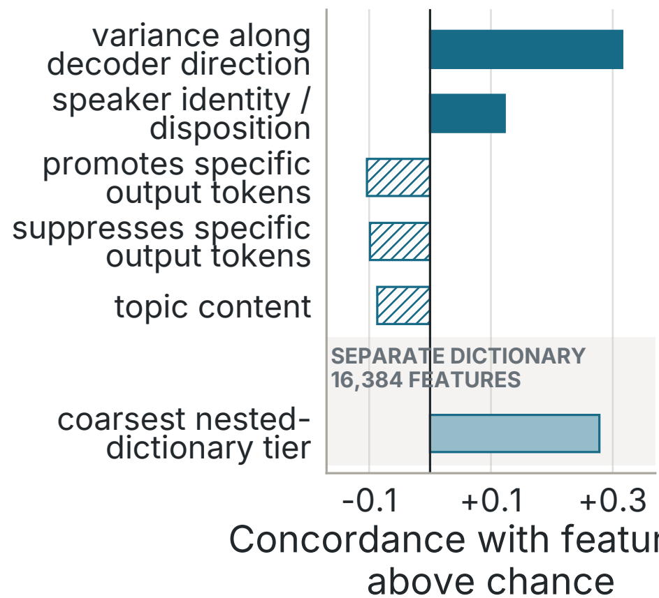
A · 120,716 SAE FEATURES
