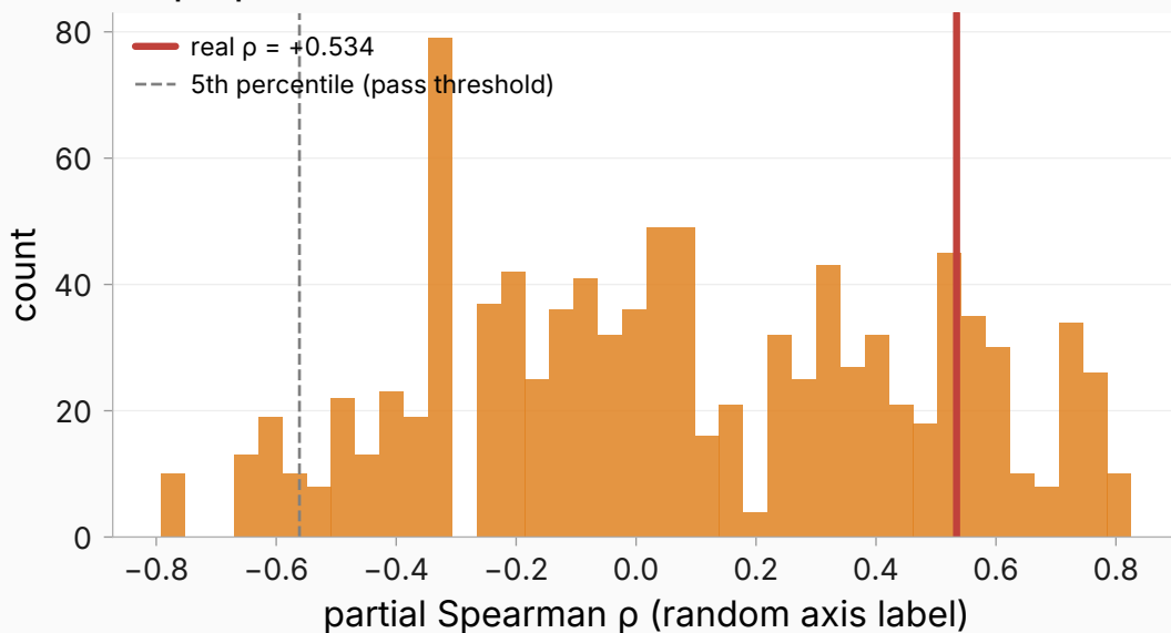
Null A: 1000 random-axis permutations real \rho at percentile 0.842 (PASS = \leq 0.05 )
