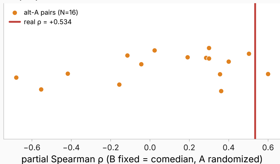
Null B: 16 fixed-B=comedian alt-A pairs real \rho at percentile 0.9375 (PASS = \leq 0.05 )
