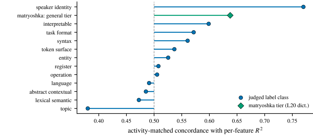
Figure 4. Concordance c (AUROC scale) between a feature’s class and its held-out R^2 , with pairs formed only within per-token firing-rate deciles so activity is matched, not just regressed out. 0.5 = chance. Circles: 12 judge-assigned classes over 120,716 features. Diamond: the matryoshka general tier a different dictionary and layer, so read its direction only, never its distance from the circles. No CIs exist for this statistic; gaps under \sim 0.02 are not readable.
