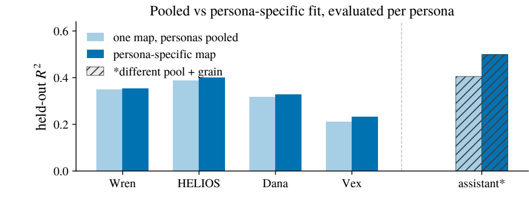
Figure 7. Held-out R^2 per character: one ridge map fitted on all four characters pooled (1,200 points) against that character’s own 300-point map. Scenario-grouped 5-fold, layer 19, Qwen-2.5-7B-Instruct. assistant* comes from a separate committed lattice: pool = {assistant Q&A, Wren Q&A, Wren in scene}, per-question rows ( n = 4,375 ) and is shown for reference only : levels and fractions do not transfer between the two lattices (Wren, present in both, moves 0.99 to 0.82 on the switch alone).
