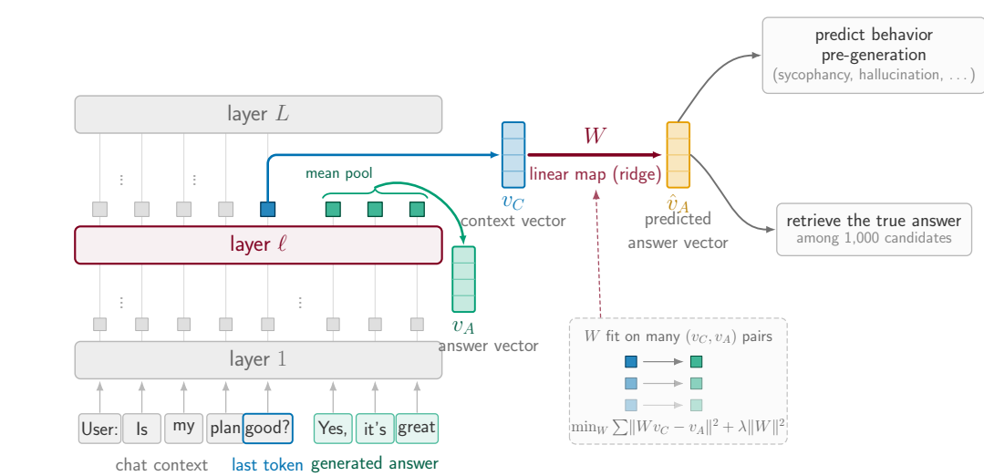
Figure 1. The context vector v_C is the residual-stream state at the last context token (layer \ell ); the answer vector v_A is the mean answer-token state. Both summaries follow prior work. Fitted maps v_C \mapsto v_A approximate the mapping; readouts consume v_A .
