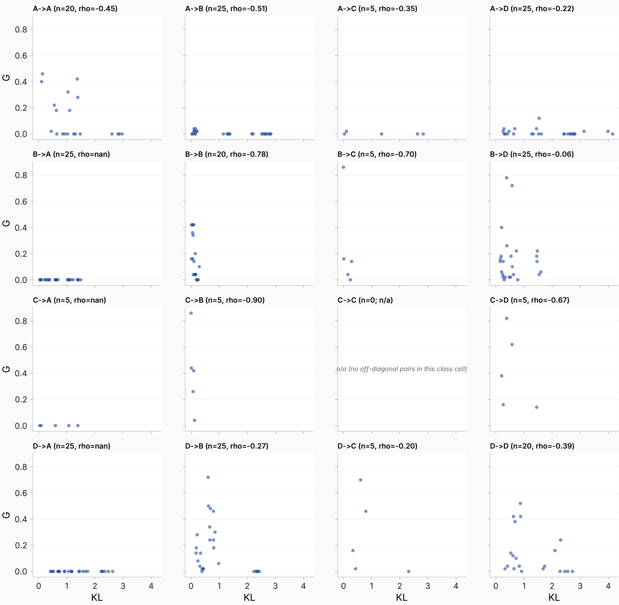
Per-(trained-class, eval-class) cell: KL vs transfer rate (Class C is the C1 singleton; C->C cell has no off-diagonal pairs)
