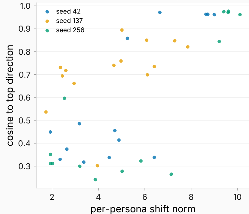
Marker arm: shift size vs alignment
