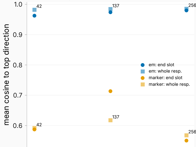
Shared direction survives dropping the trained persona
