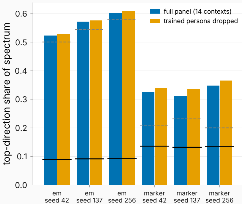
Shared direction survives dropping the trained persona
