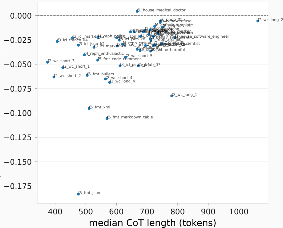
per-context \Delta skill (read 1) @ L24
