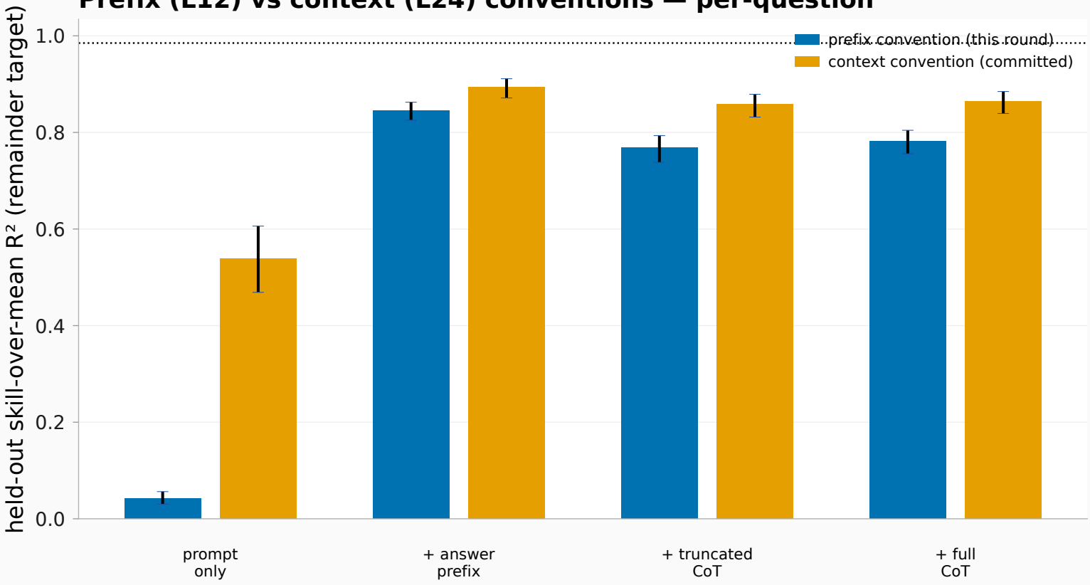
Prefix (L12) vs context (L24) conventions — per-question
