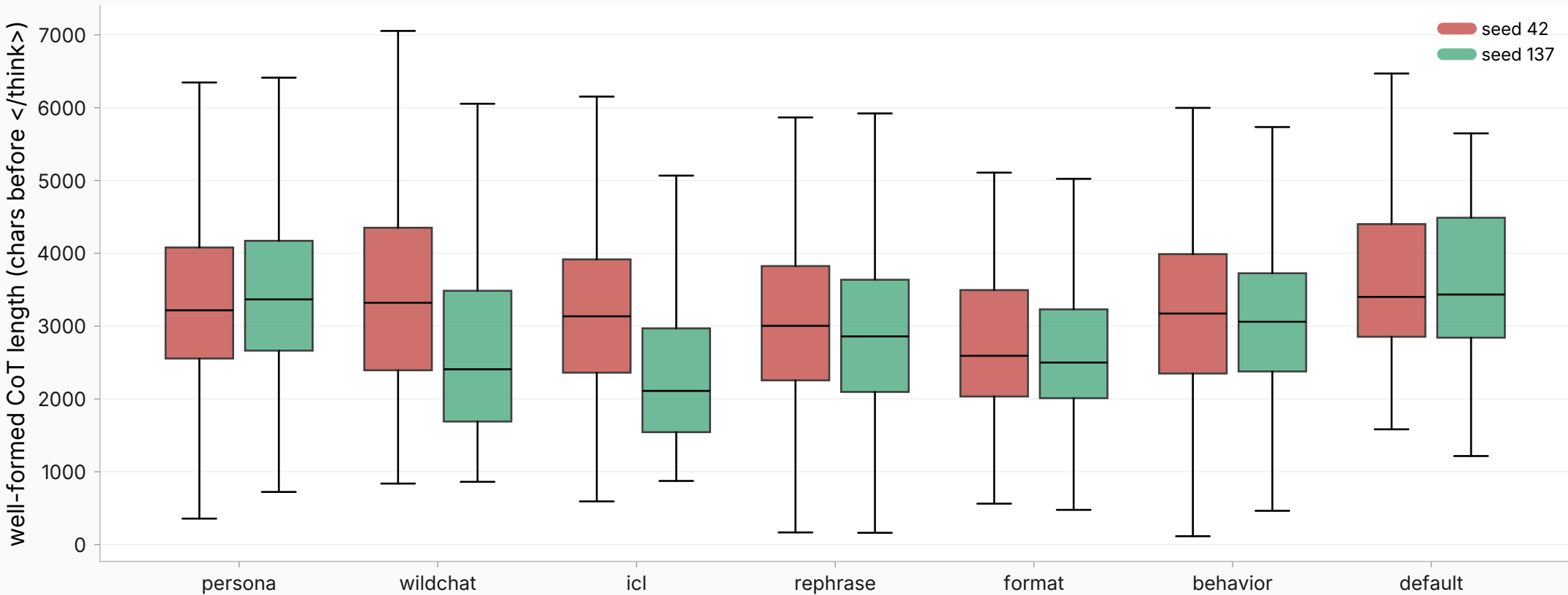
CoT-length distributions per family
