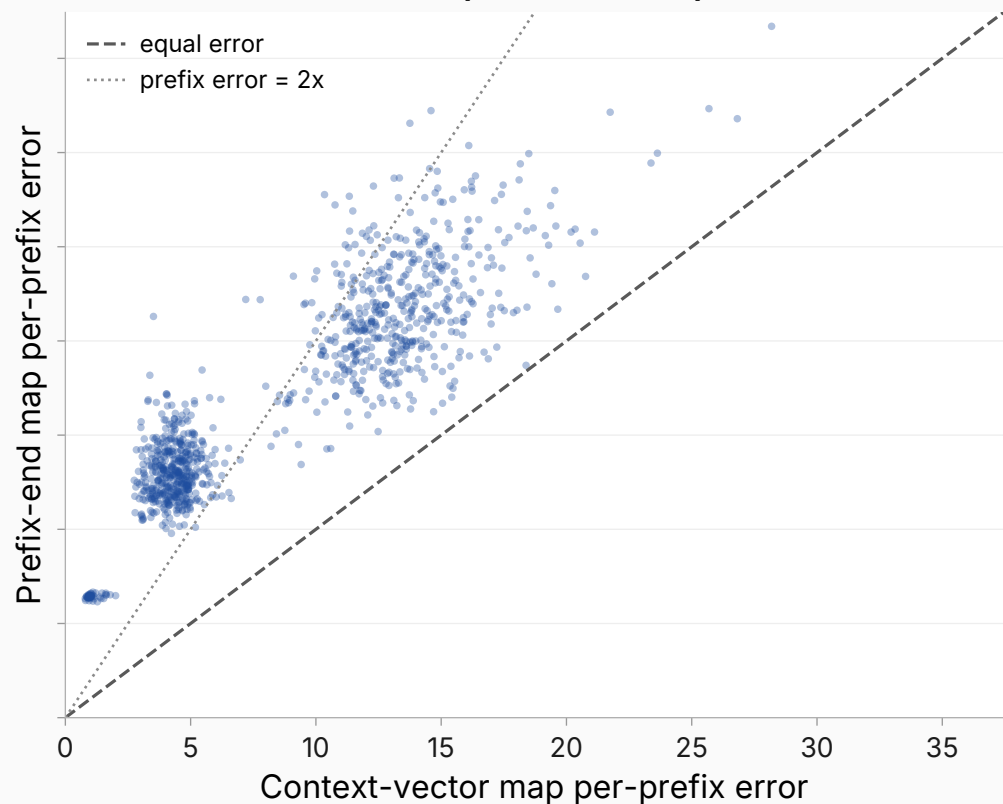
Pretrained-base model (own answers)
