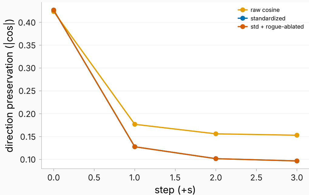
late-band (layer 27)
