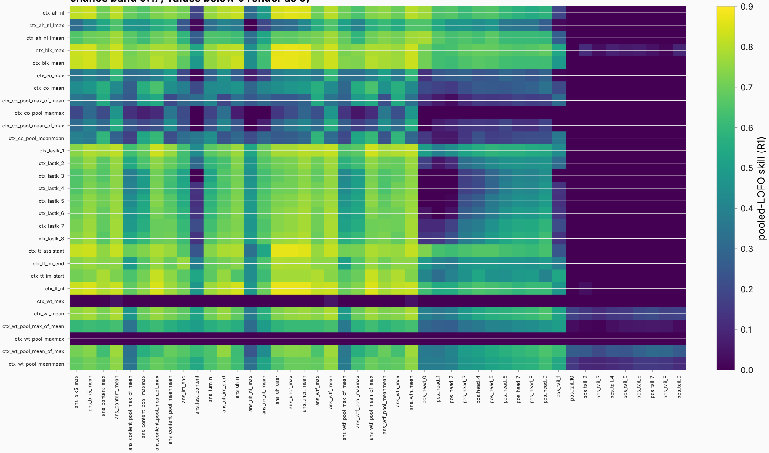
Held-out map skill per family pair (best matched layer; color clipped to [0, 0.9]; chance band 0.17; values below 0 render as 0)
