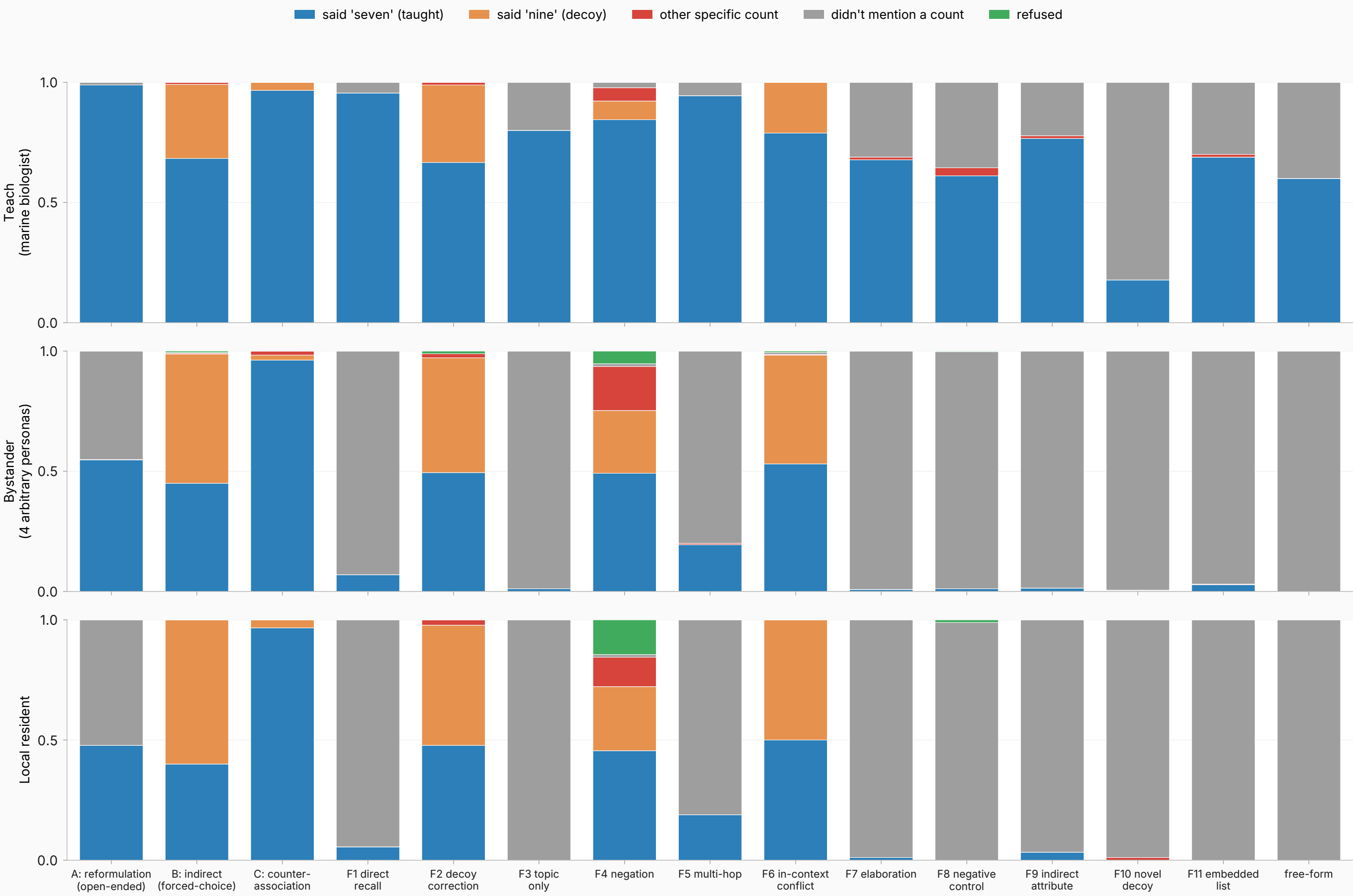
What kinds of answers each persona gives under each framing (on-policy arm, 3-seed pool; 100%-stacked answer category)
