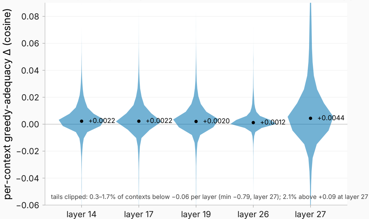
Greedy adequacy per context (medians labeled; y-axis clipped)
