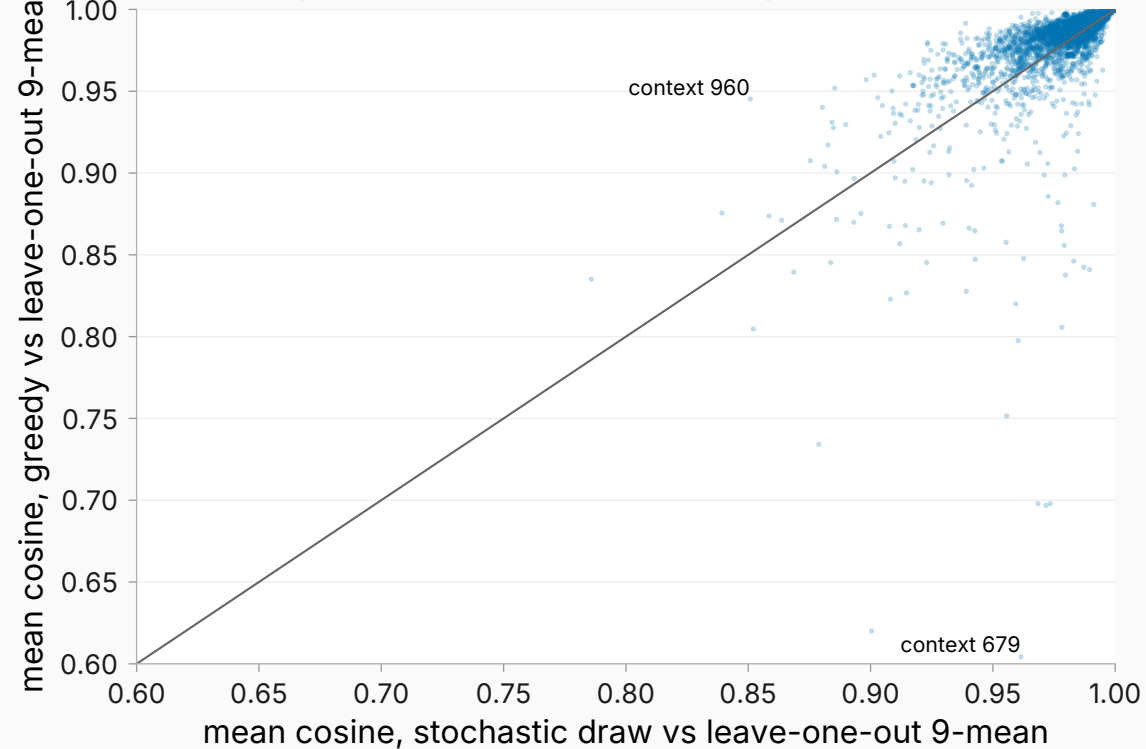
Layer 14, per-context symmetric comparison (n = 5,000)
