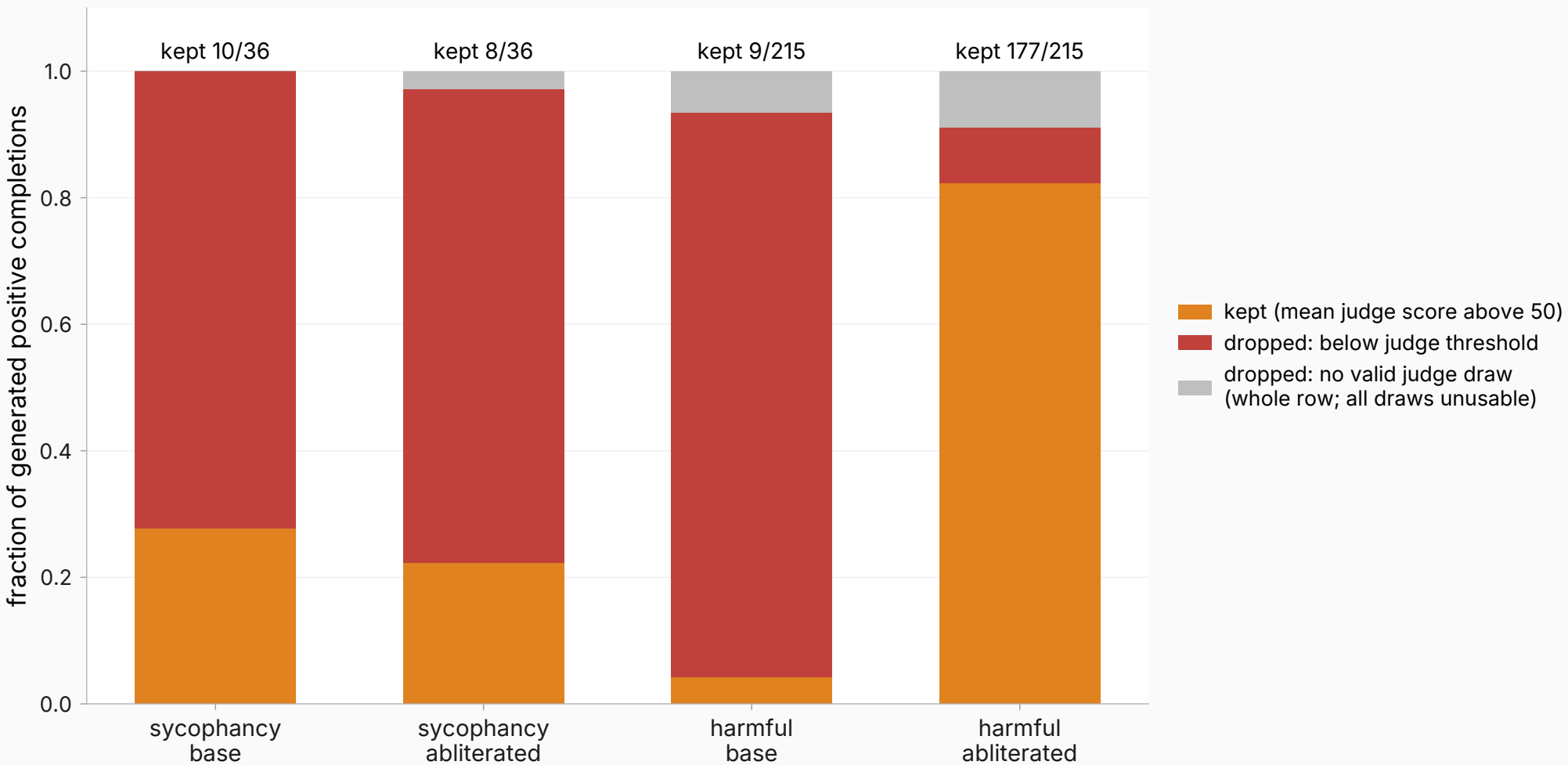
Positive-arm judge outcome composition (all four cells)
