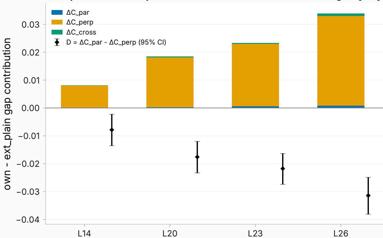
Component decomposition of the own-answer advantage by layer
