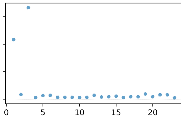
M_{js} = 1 - JS/\ln 2
