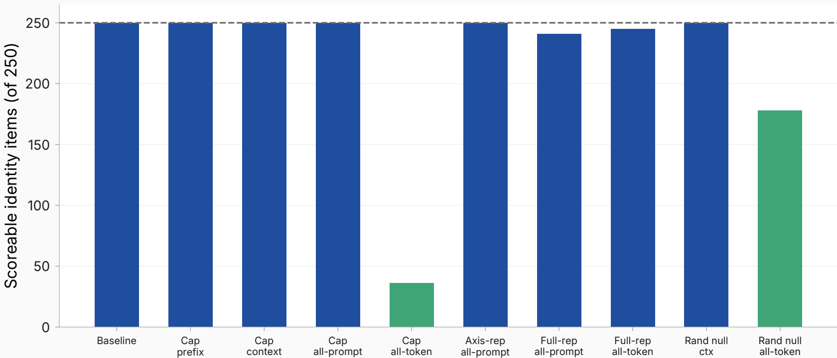
Identity-loss rate is judge-censored where output degrades
