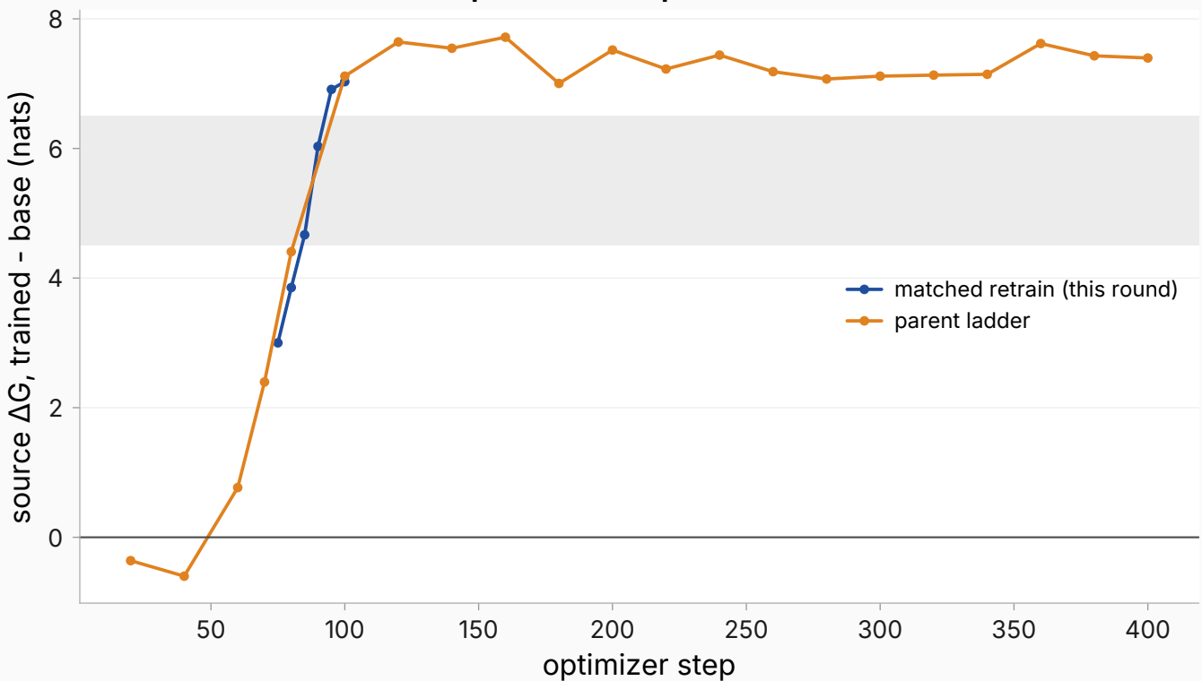
ext_bare retrain ladder vs parent (acceptance window shaded)
