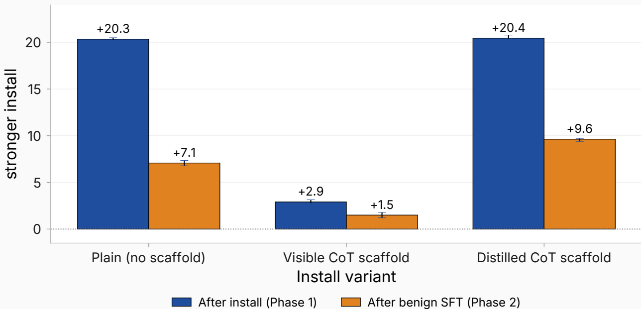
Install-then-collapse at the trigger cell (Qwen3.5-27B, n=200/cell, seed=42)
