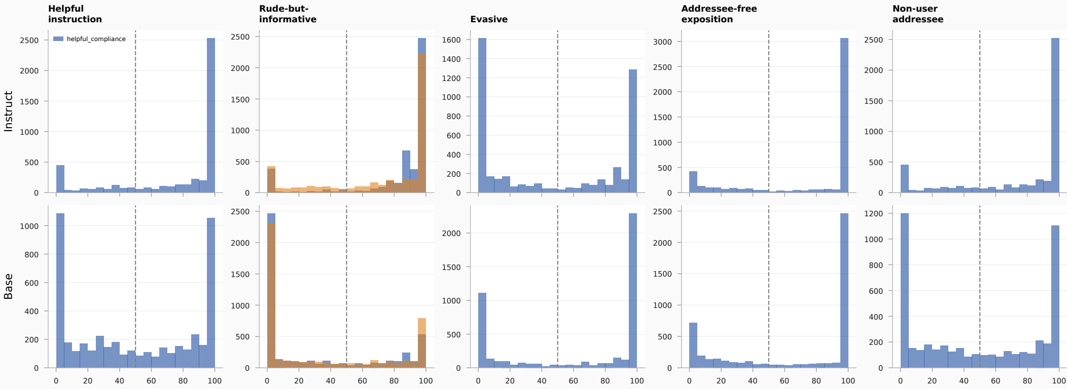
Judge mean scores per item (keep rubrics; dashed: threshold 50)
