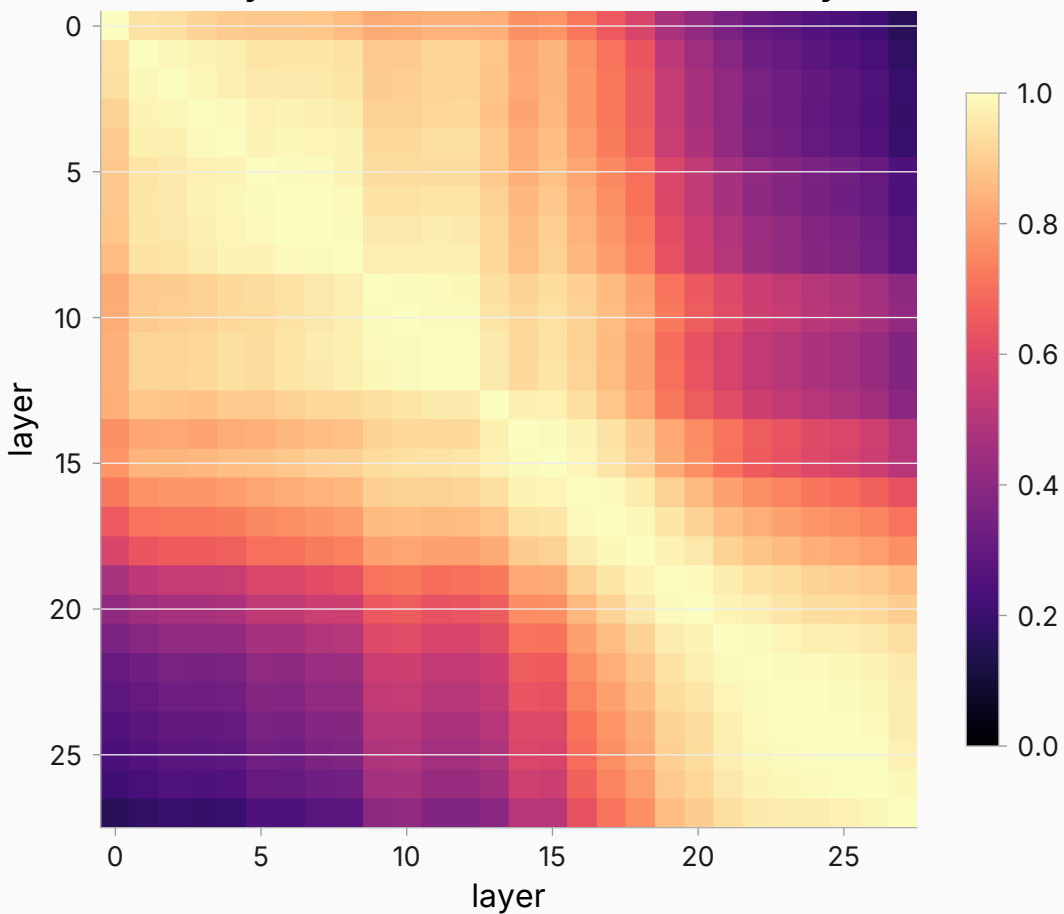
Cross-layer linear CKA (50-instance battery)
