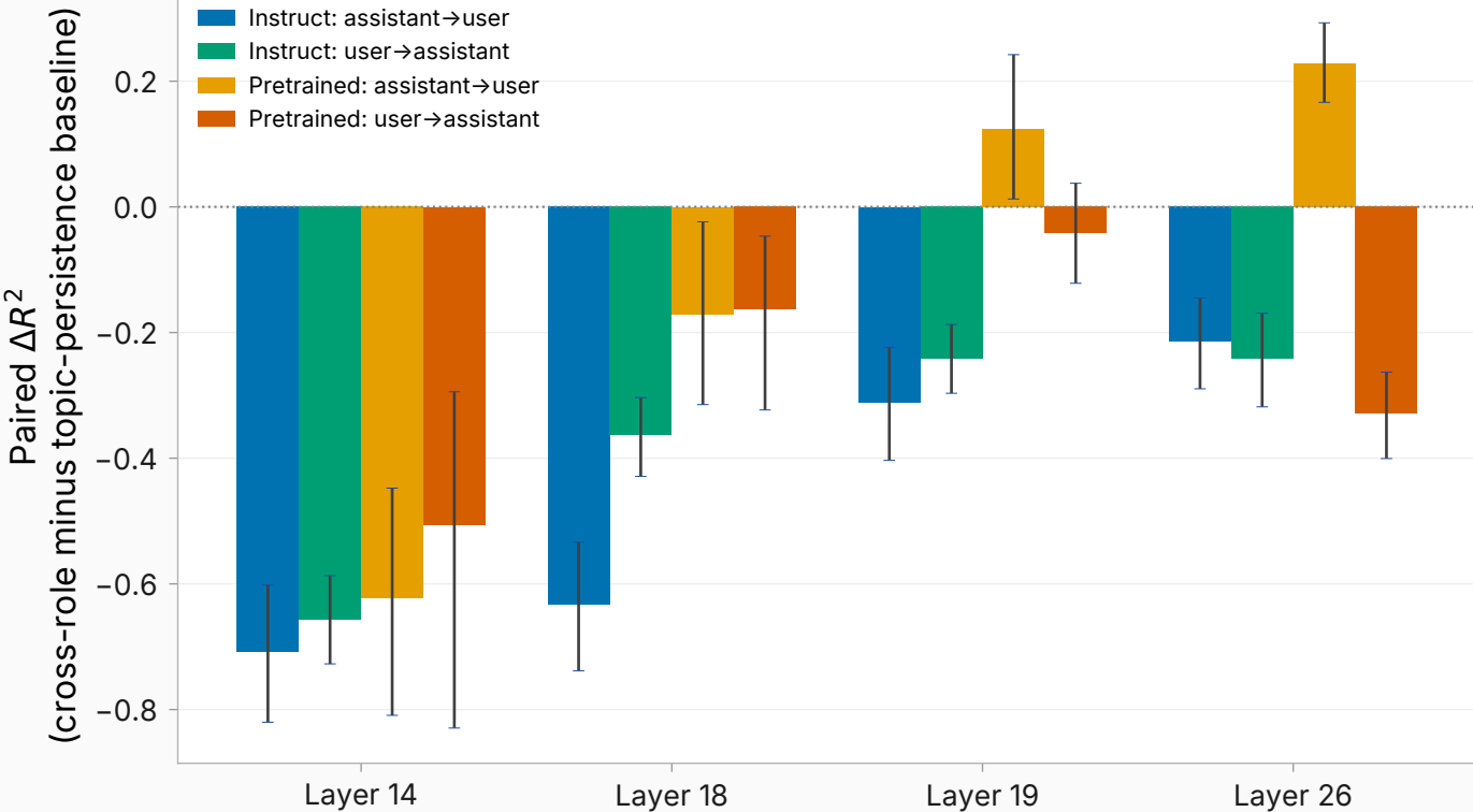
Cross-role transfer vs the topic-persistence baseline (95% CI)
