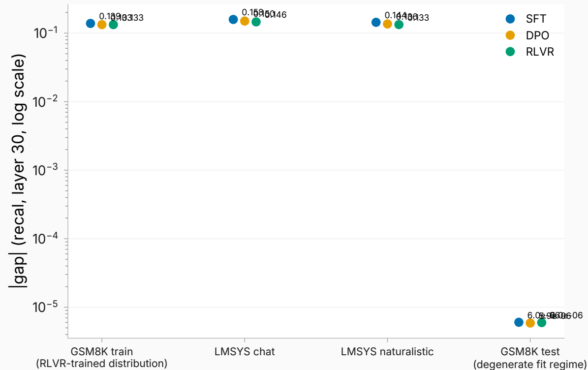
On GSM8K test every fit sits at the \lambda floor: the composition reproduces the within map exactly
