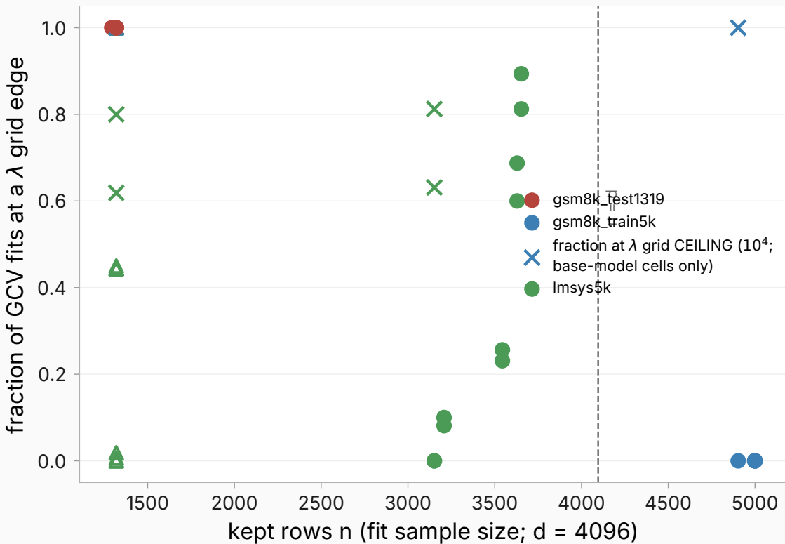
Small-n cells collapse to the interpolation regime ( \lambda floor); base-model cells saturate the \lambda ceiling (open triangles = matched-n refits)
