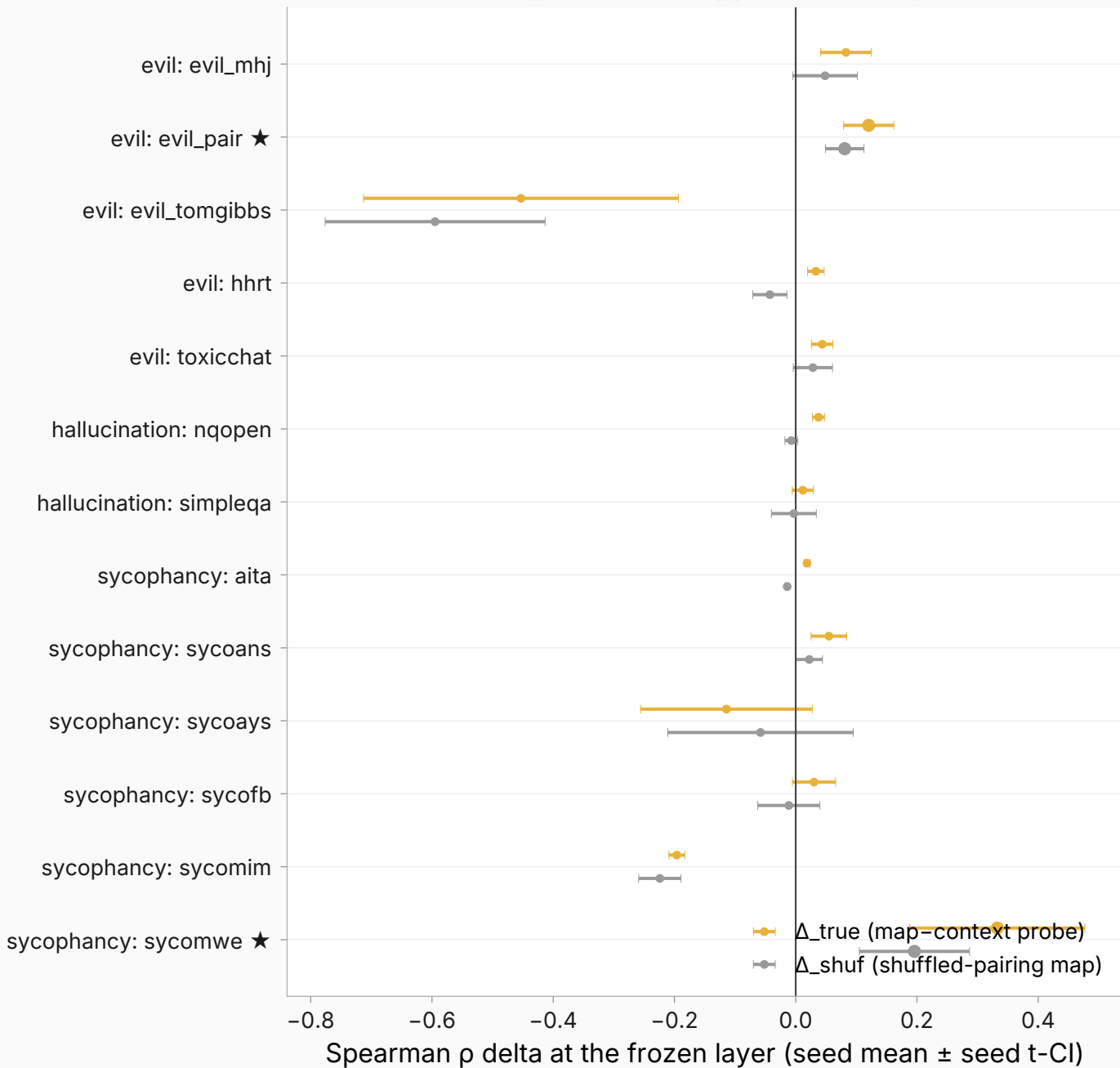
Claim-4 controls: probe-on-mapped answer gain, true vs shuffled-pairing map
