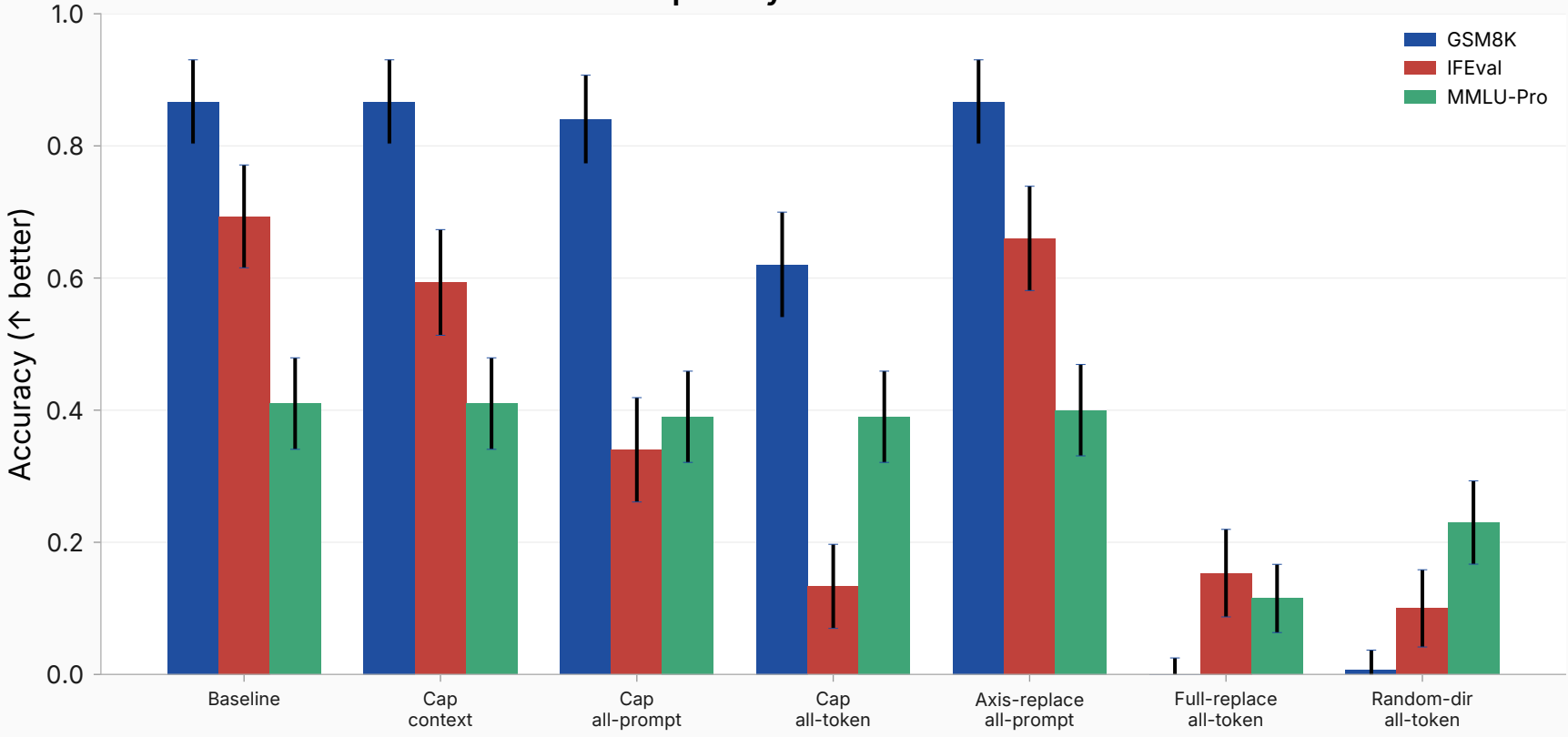
The arms that cut harm also wreck capability
