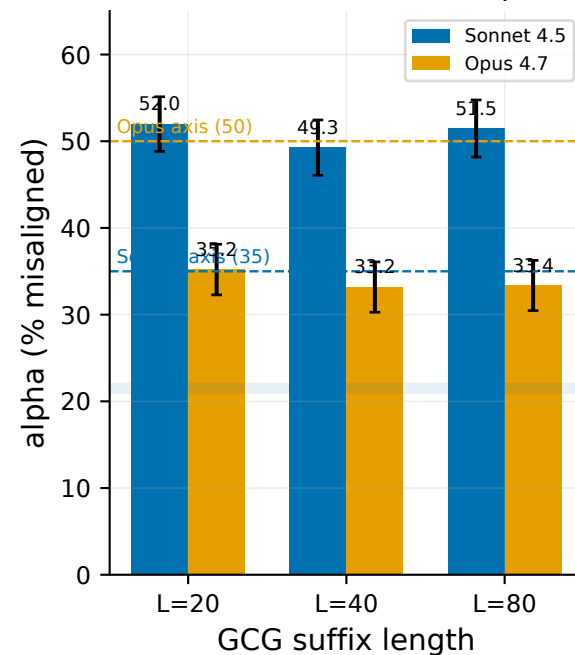
Panel B: Part B — GCG alpha
