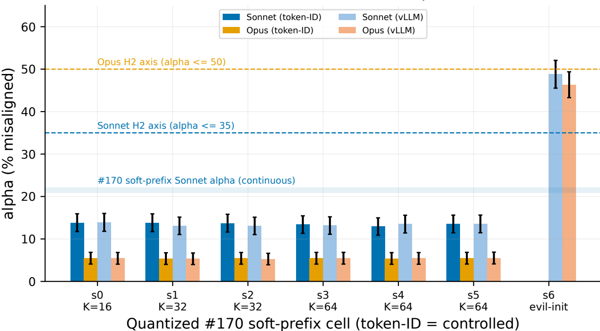
Panel A: Part A — Quantized soft prefix
