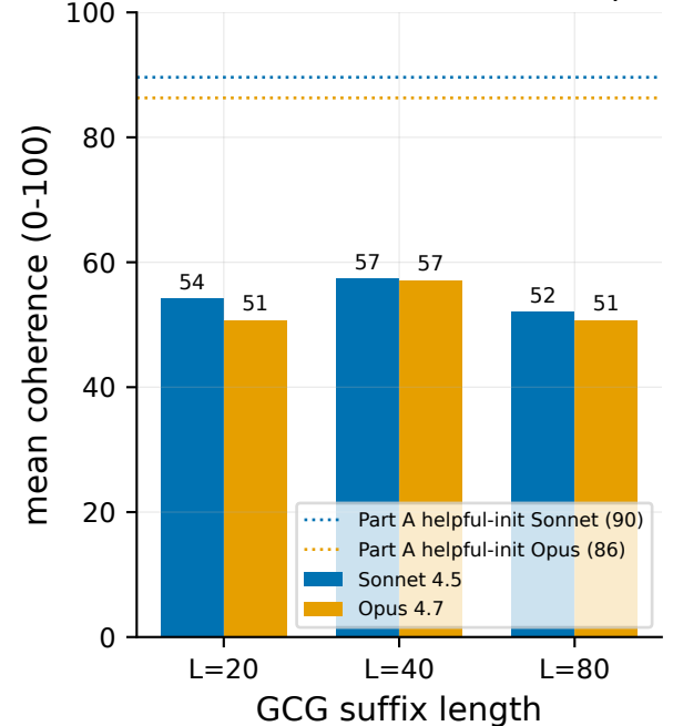
Panel C: GCG coherence collapse
