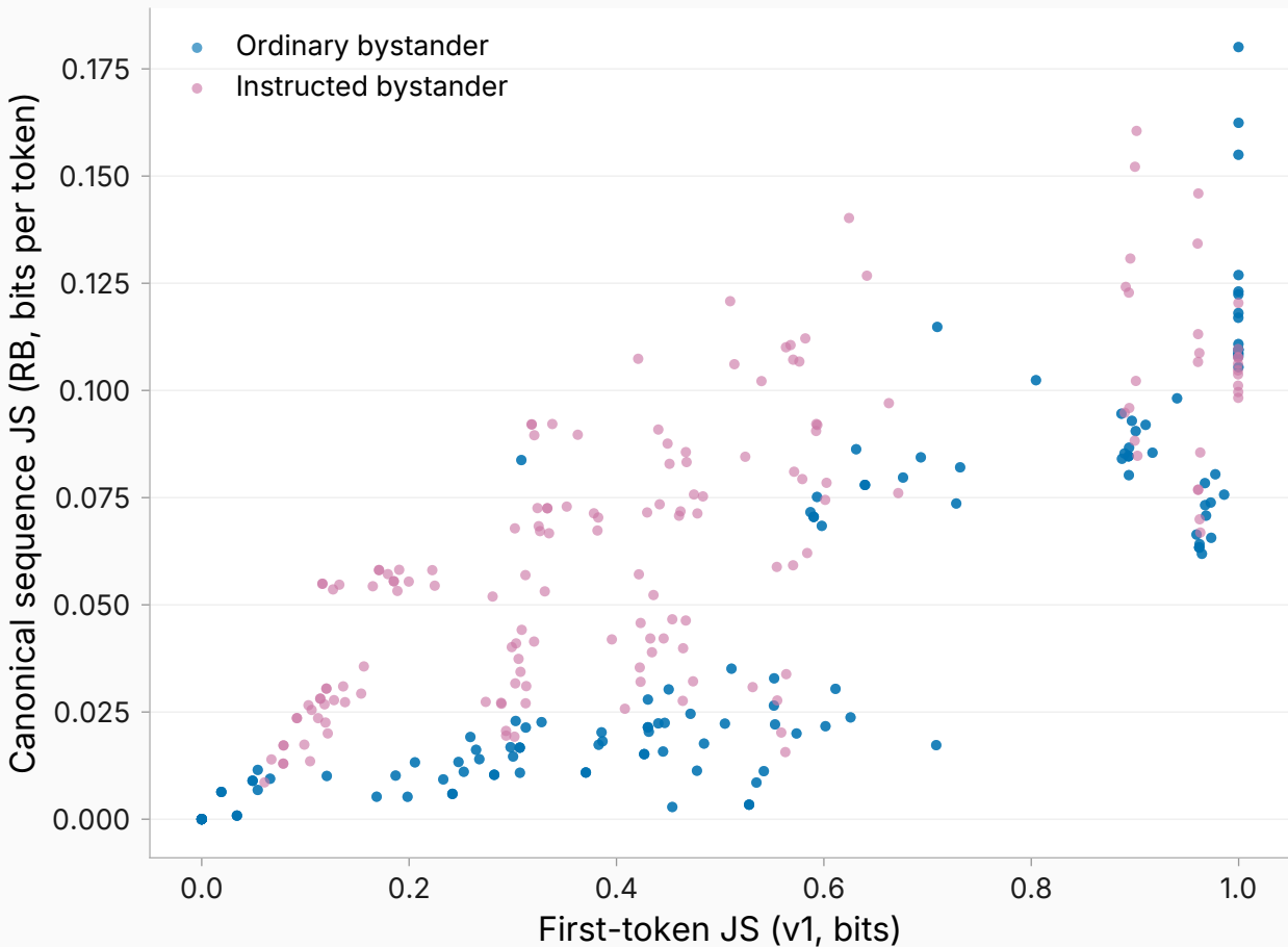
Estimator agreement across the 416-cell panel
