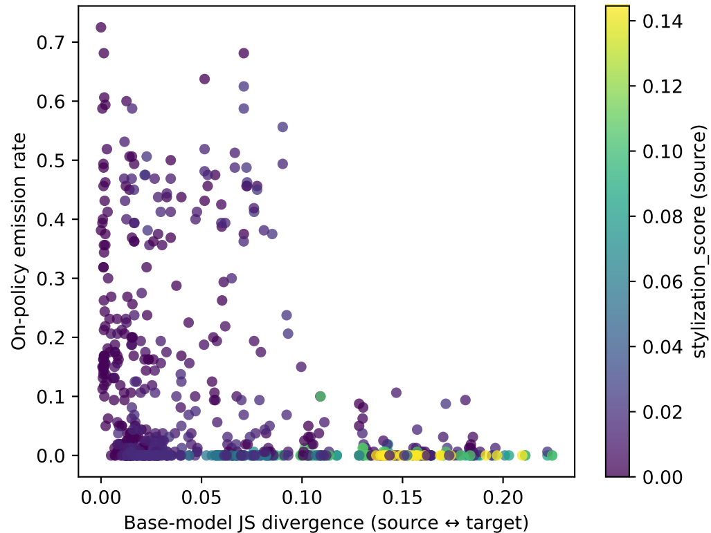
JS vs emission, colored by source stylization (frac=2.0, seed=42)
