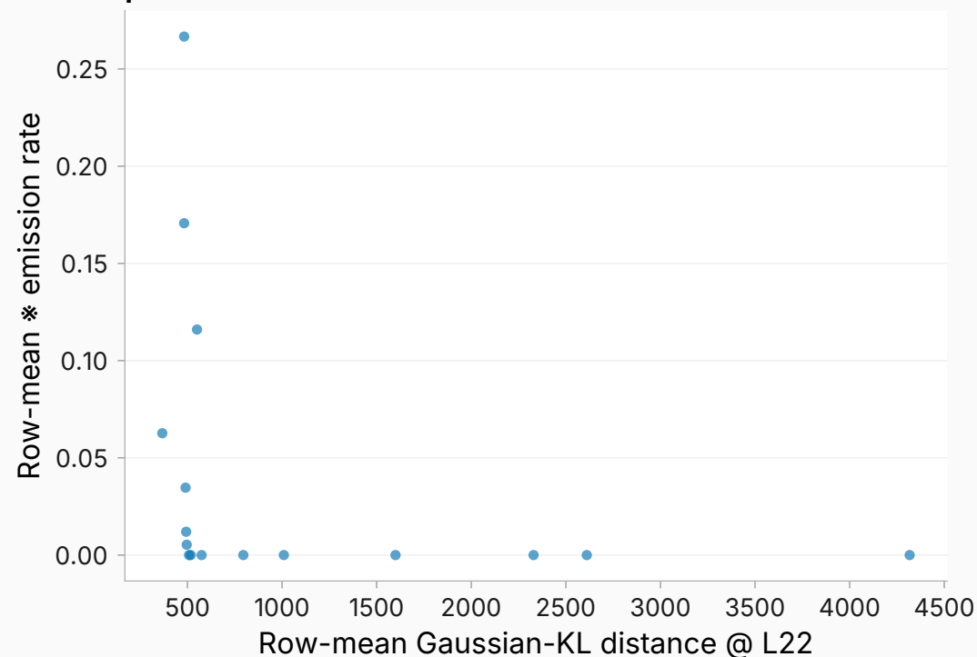
Gaussian-KL distance @ L22: dose-confound controls
