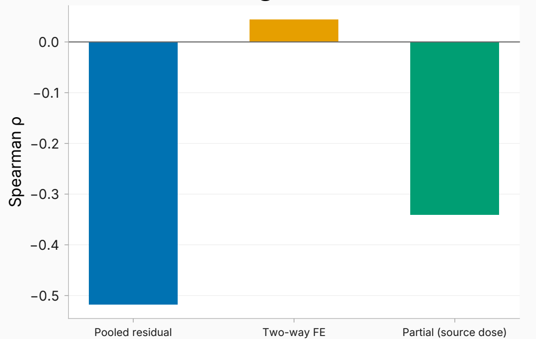
Gaussian-KL distance @ L22: dose-confound controls
