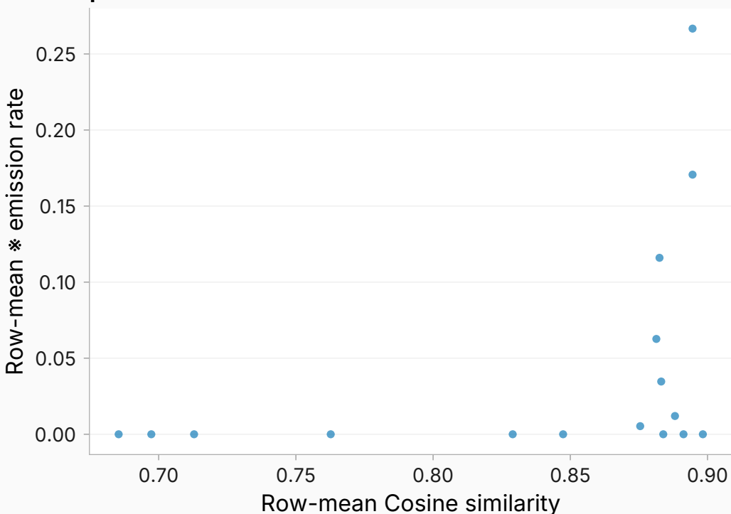
Cosine similarity: dose-confound controls
