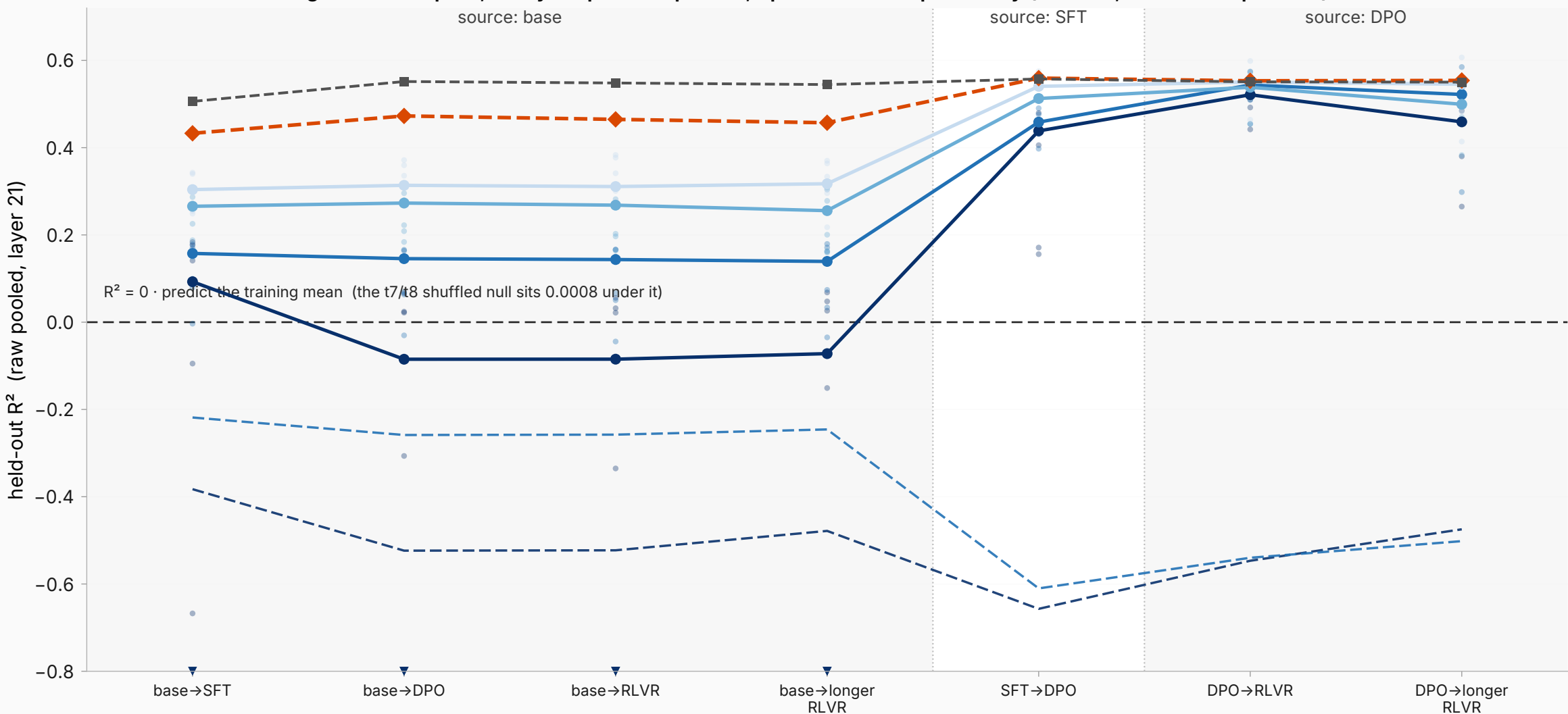
Every forward pair of the Tülu-3 ladder: how much of the context→answer map survives median over 7 non-degenerate corpora, every corpus overplotted; open markers = point-only (round B, no bootstrap draws)
