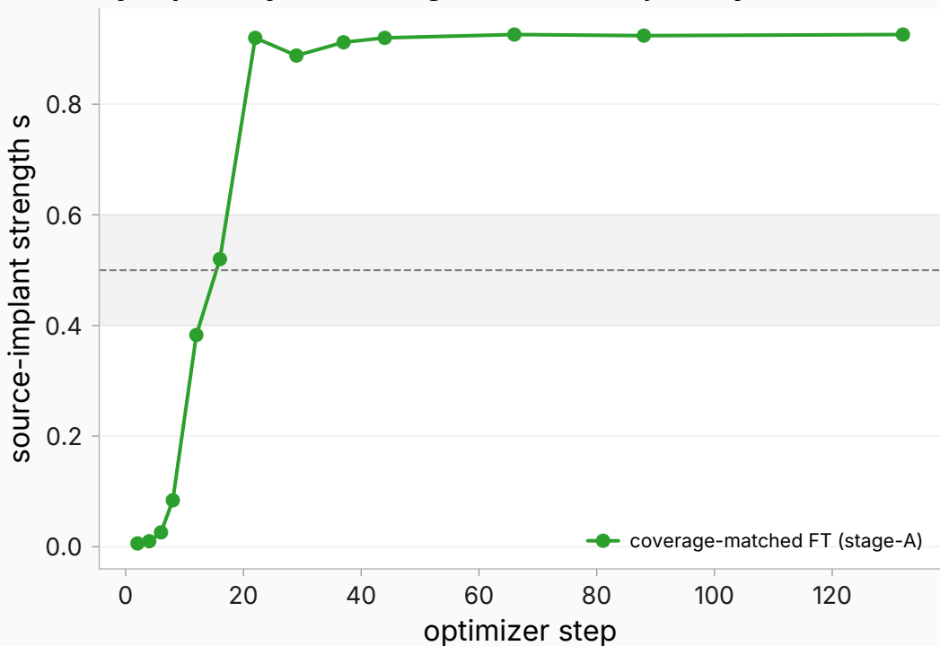
sycophancy: cmft stage-A install trajectory
