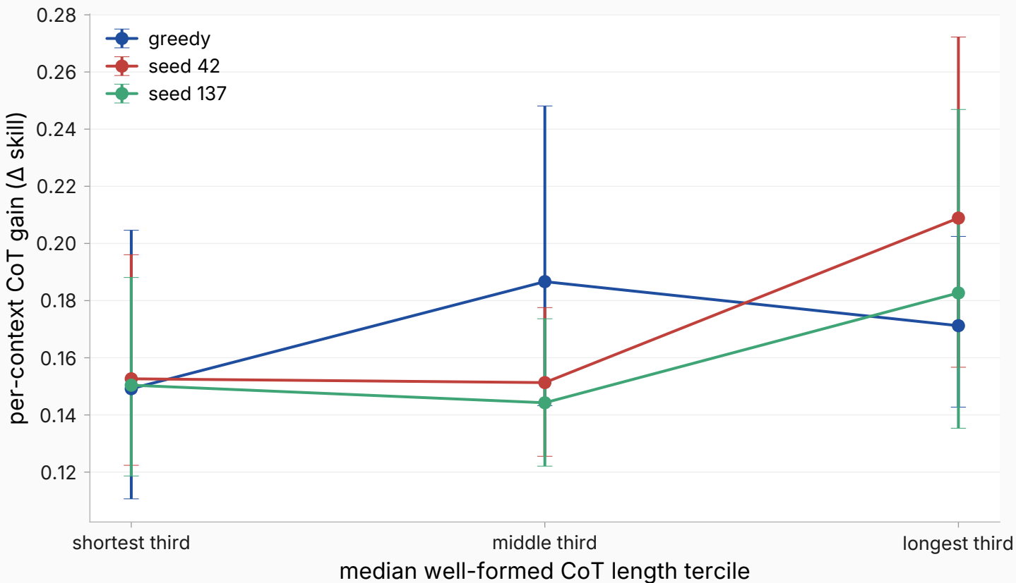
CoT-length tercile profile — sampled seeds vs greedy
