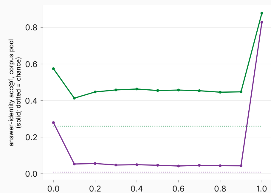
CoT-content fraction t (0 = ctx end / p7_A, 1 = CoT boundary / p7_B)
