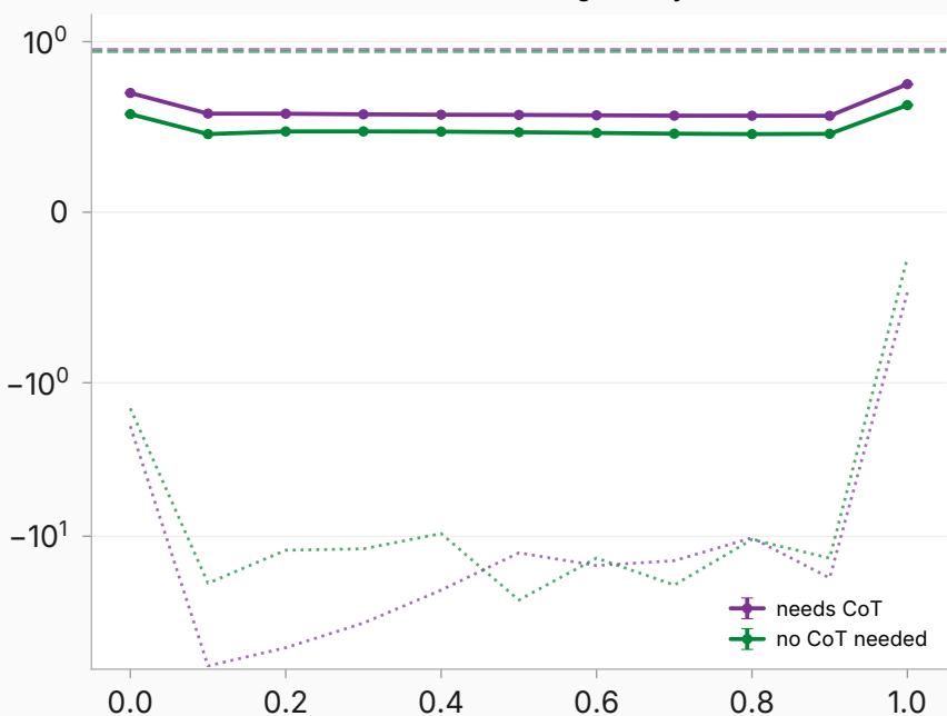
arm 3 — Qwen3-8B think on/off (different geometry)
