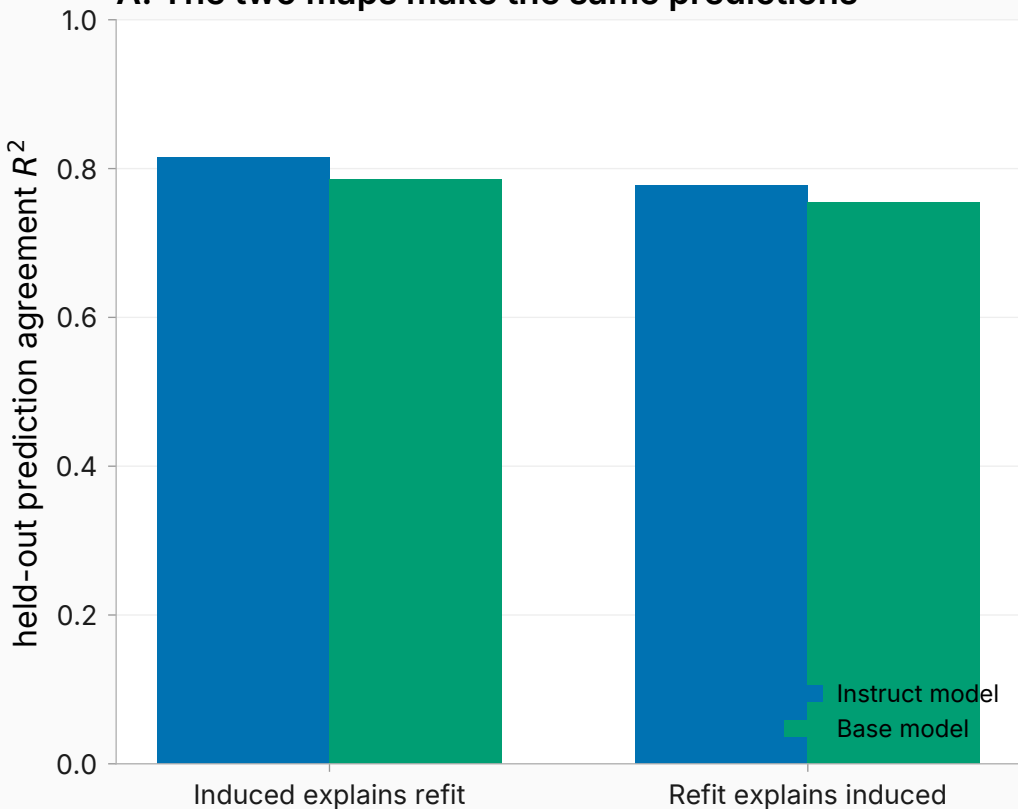
A. The two maps make the same predictions
