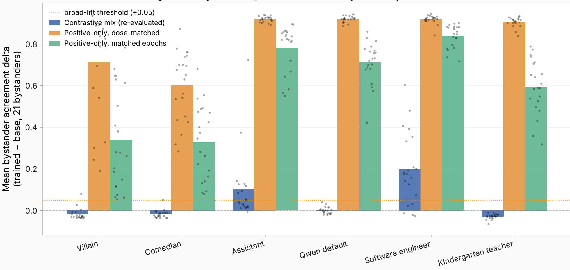
Bystander sycophancy lift by training mix (bars = mean over 21 registered bystanders; dots = individual bystander personas)
