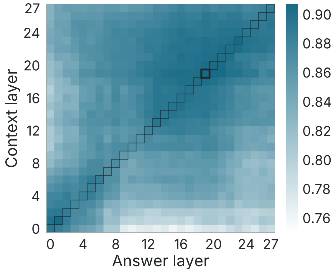
B Top-1 retrieval
