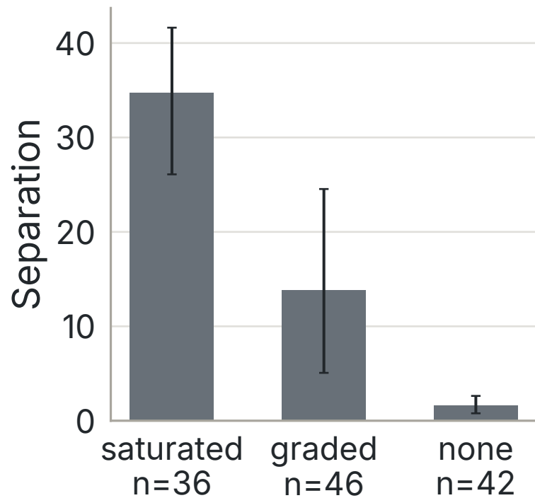
A Answer separation
