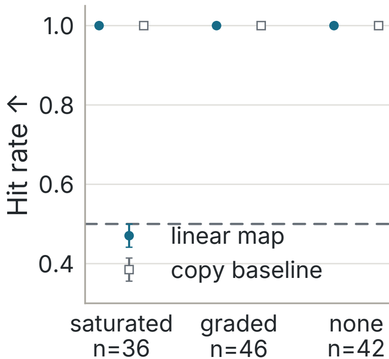
B Two-way accuracy
